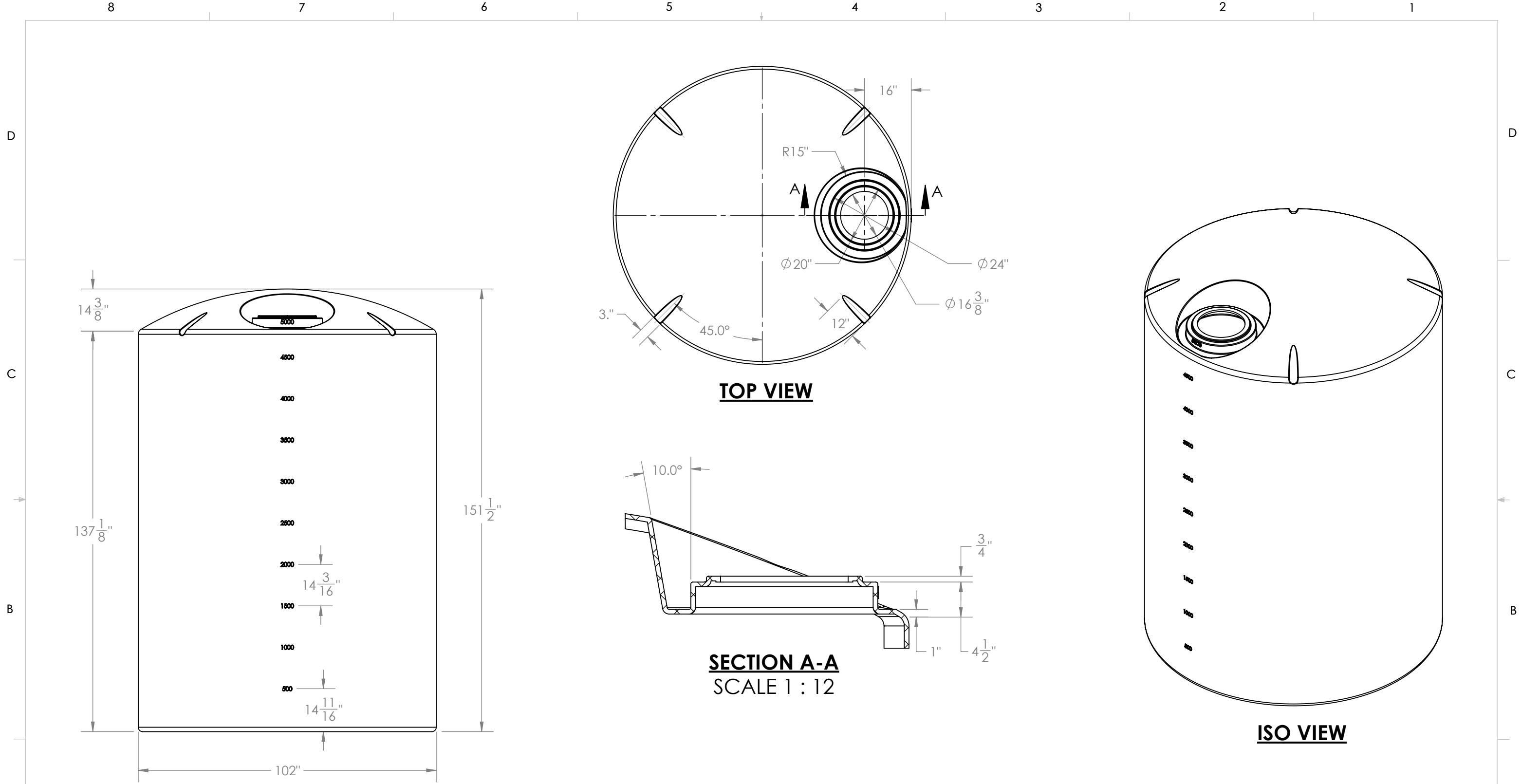
FRONT VIEW
