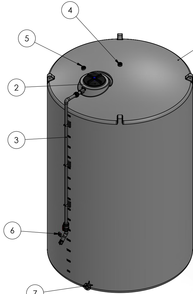
ISOMETRIC VIEW (FRONT)
