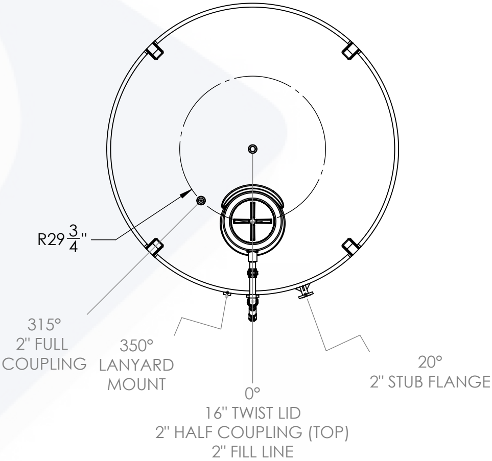
PLAN VIEW
