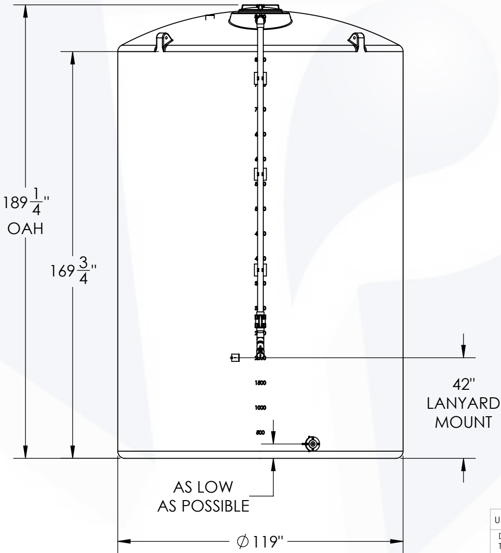
FRONT VIEW
