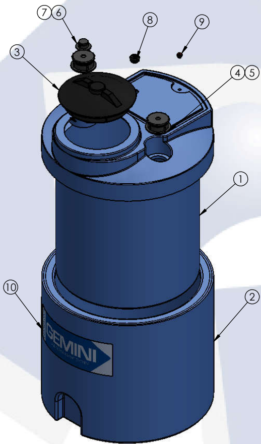
ISOMETRIC VIEW (EXPLODED)
