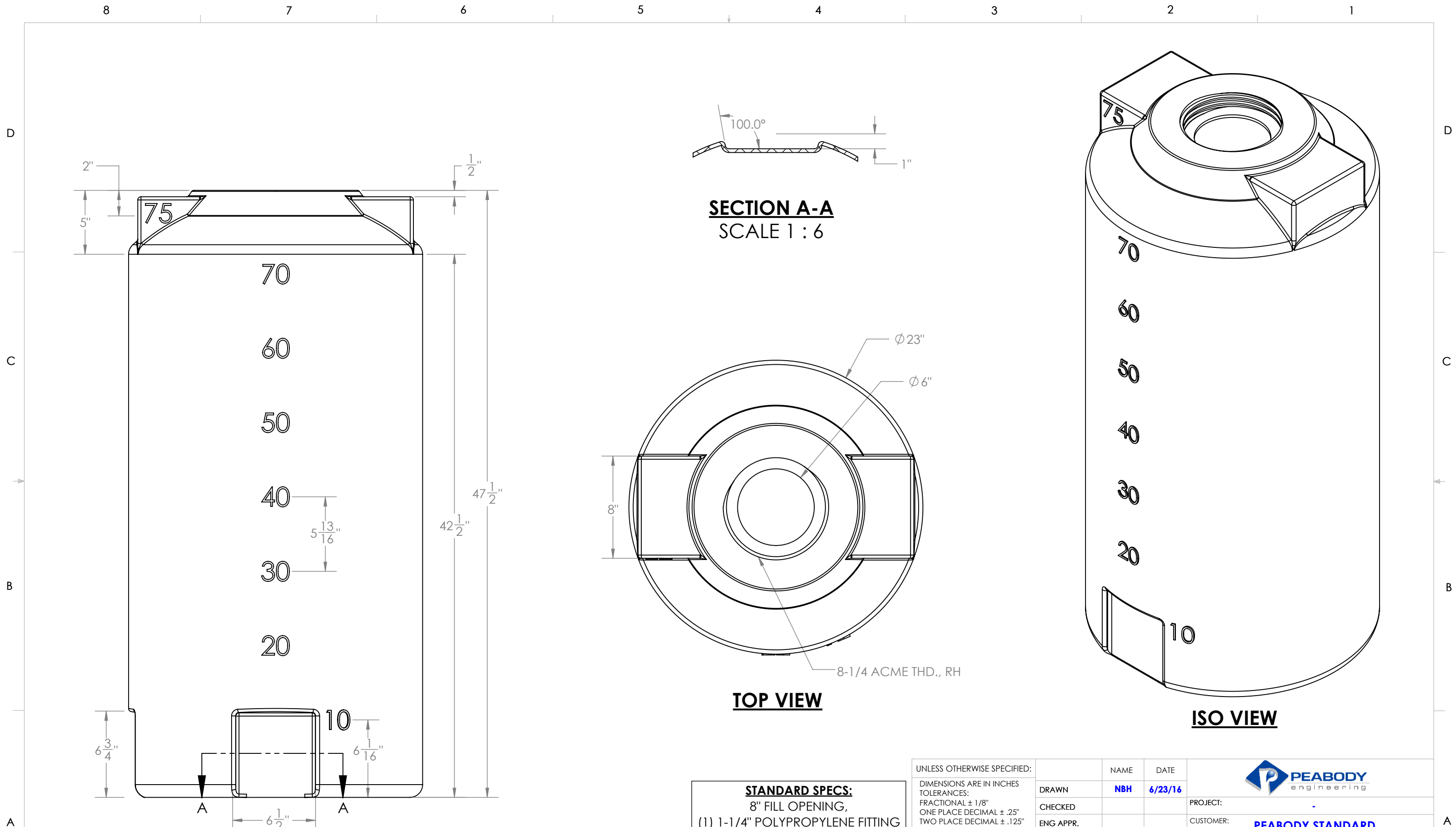
FRONT VIEW
