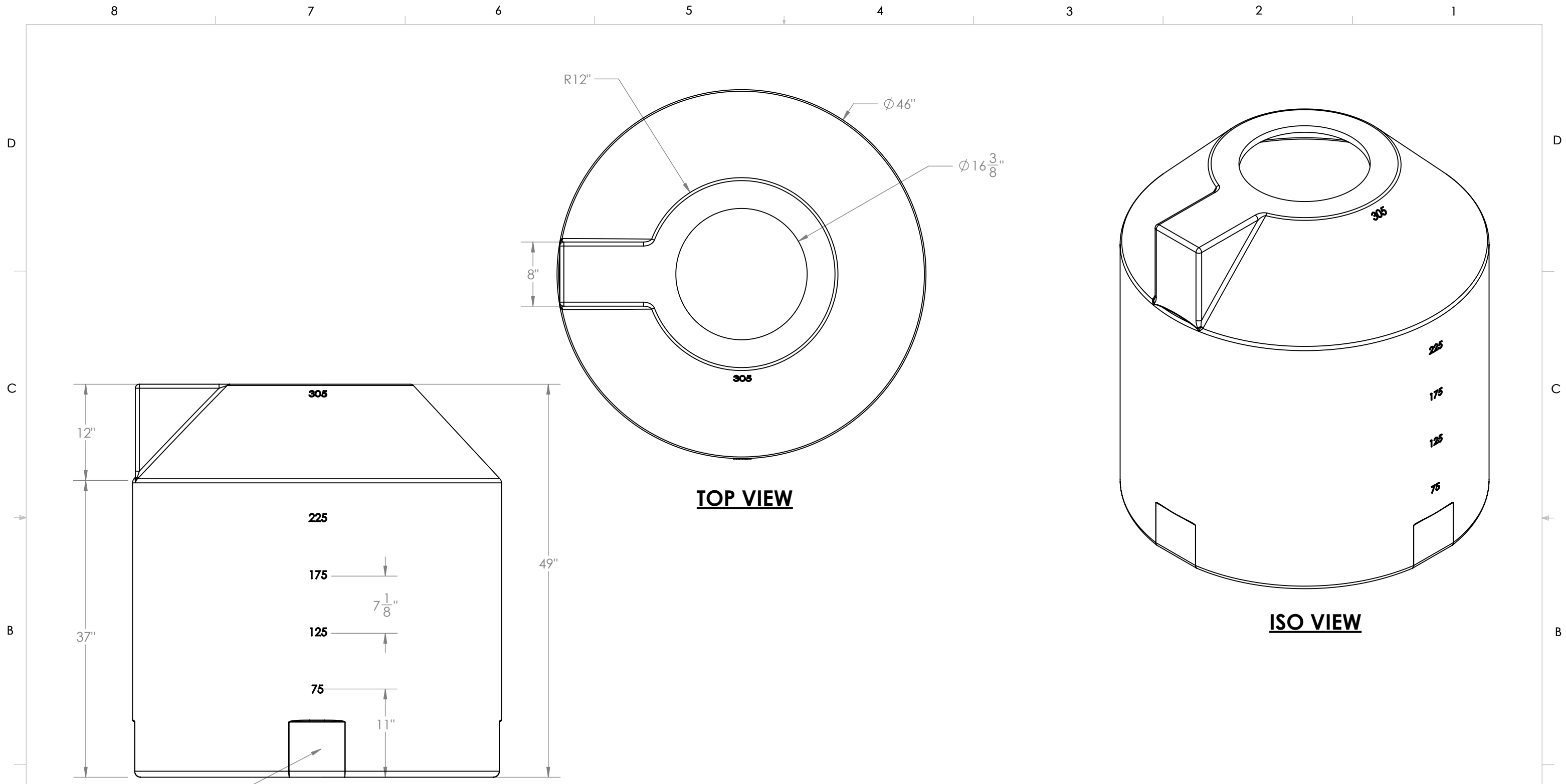
FRONT VIEW
